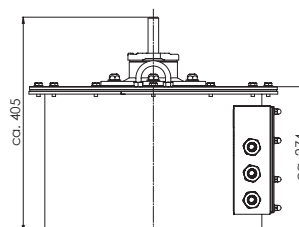
Remote Unit for SS350 and SS450
