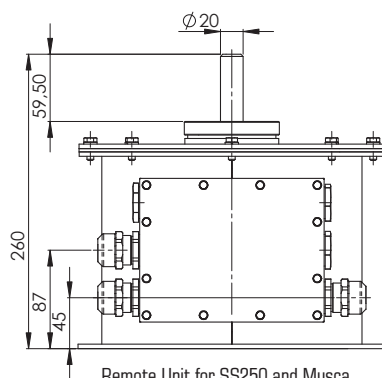
Remote Unit for SS250 and Musca
