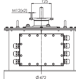
Remote Unit for SS350 and SS450 with Searchlight
